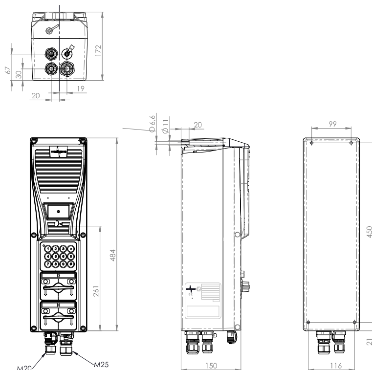
Fig. 1: Dimensional drawing 4 DXE 715
