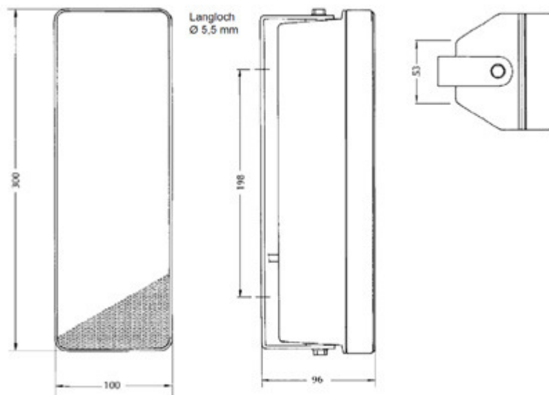
Fig. 1: Dimensional drawing AL 10-T12 EN54
