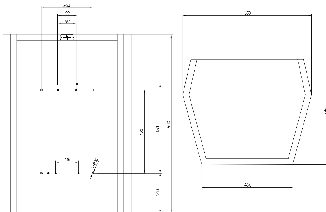
Fig. 2: Dimensional drawing 2 SSH 15
