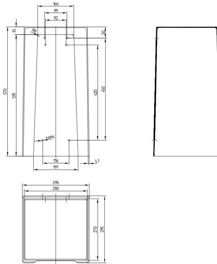
Fig. 1: Dimensional drawing 1 SHX 05
