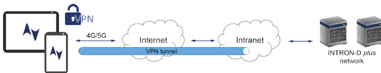
Fig. 2: Connect the DUSTRON to a Public 4G/5G Mobile Network
