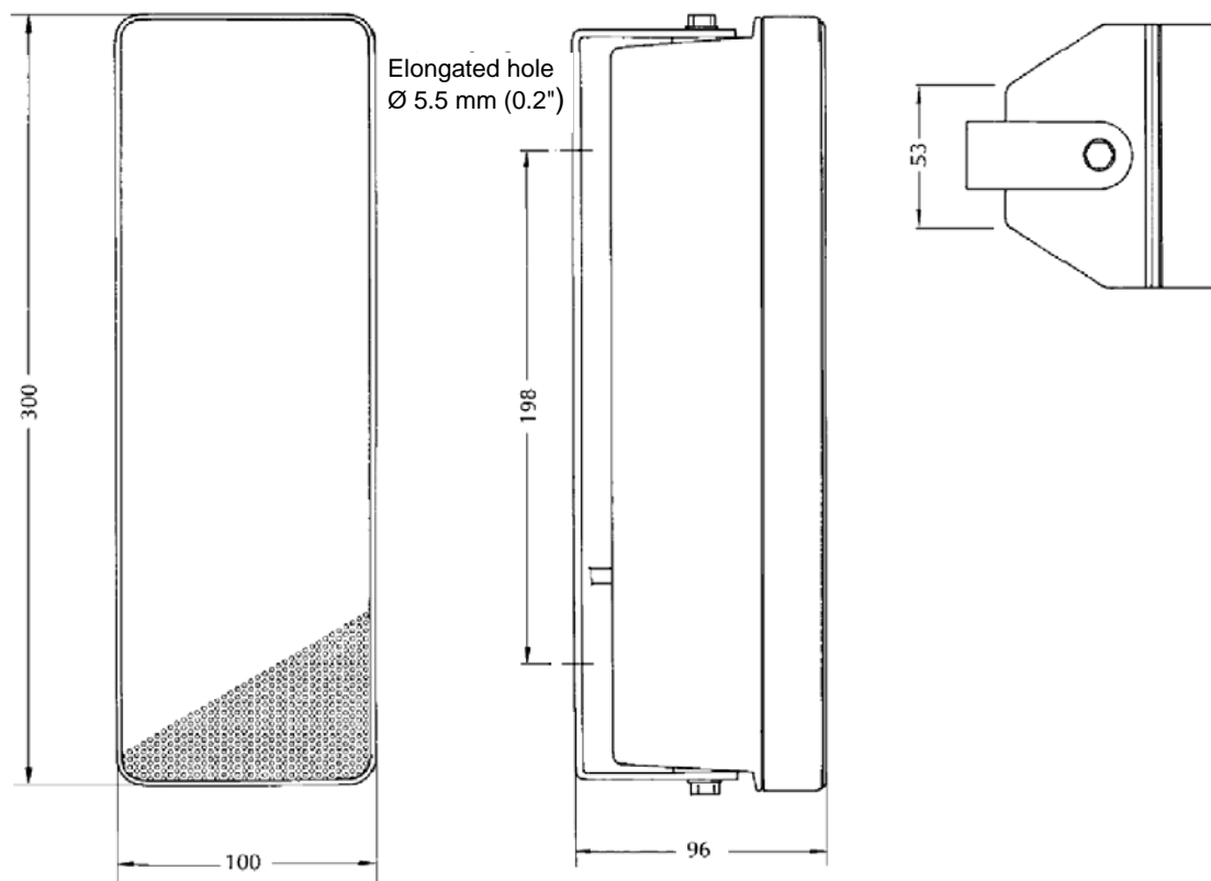
Fig. 1: Dimensional drawing AL 10
