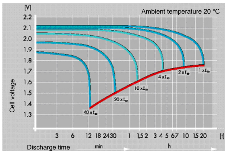
Fig. 1: Discharge characteristics 4 NSV
