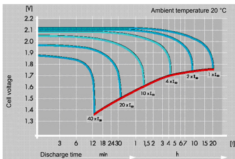
Figure 1: Discharge characteristics 4 NSV
