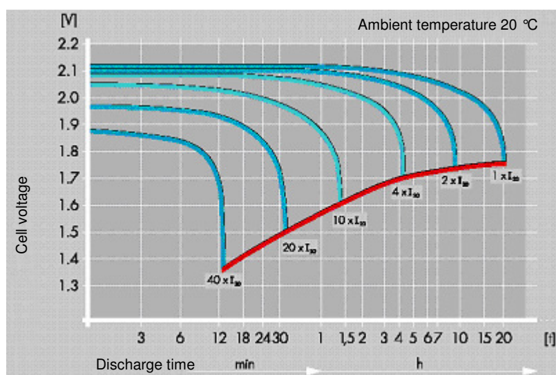
Figure 1: Discharge characteristics 5 NSV
