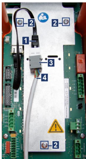
Fig. 14: NRO 0x2 with one Ethernet interface
