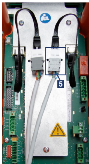
Fig. 15: NRO 1x2 with two Ethernet interfaces
