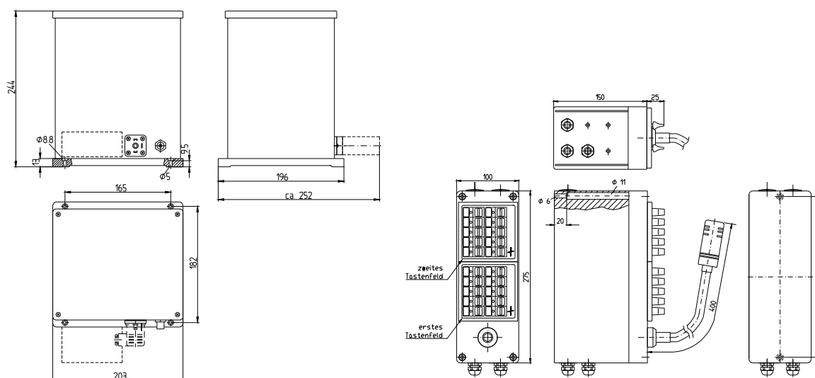
Figure: Dimensional drawing 20 / 32 FKUH 10 respectively 20 / 32 FKVH 10
