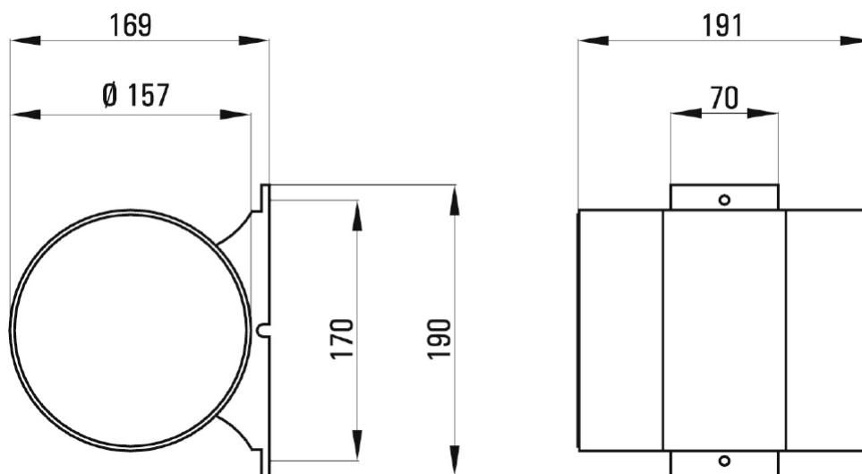
Figure 1: Dimensional drawing LWD 12 Ü
