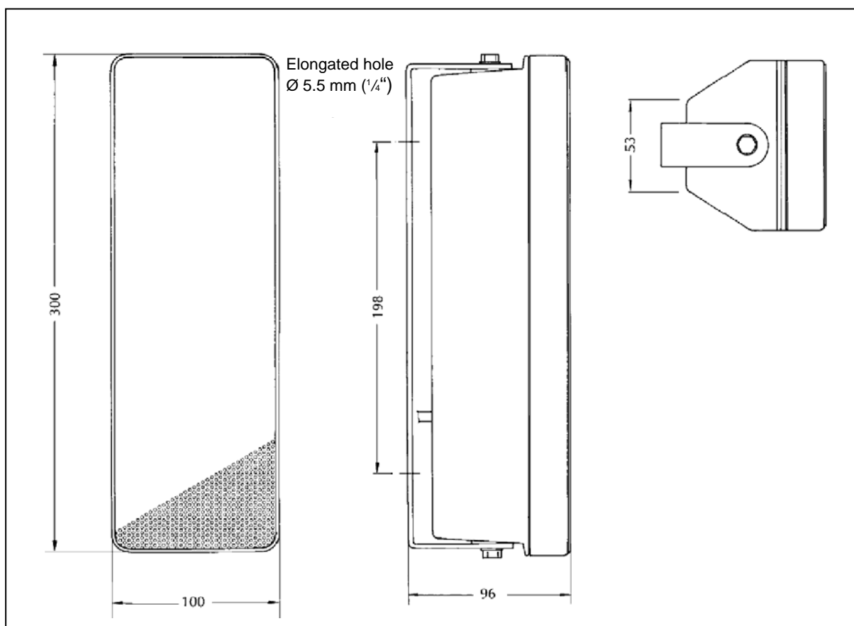
Figure 1: Dimensional drawing AL 10
